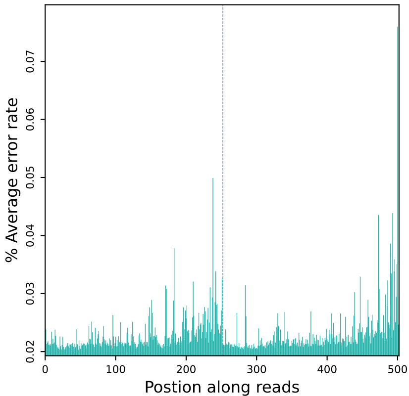
Error rate distribution along reads (R10416)
